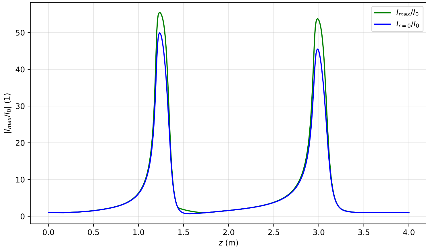
I_{max}(x=0, y=0, z)/I_0 , \text{Pin}=1.9\text{Pcr} , noisy input, artificial time
